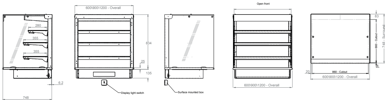
End Elevation Rear Elevation End Elevation Front Elevation Plan
