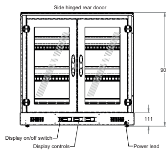
Rear Elevation
