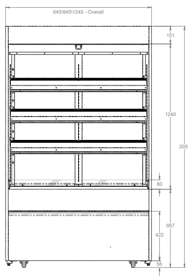
Front Elevation
