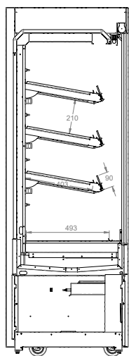
Section Elevation
