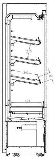
Section Elevation
