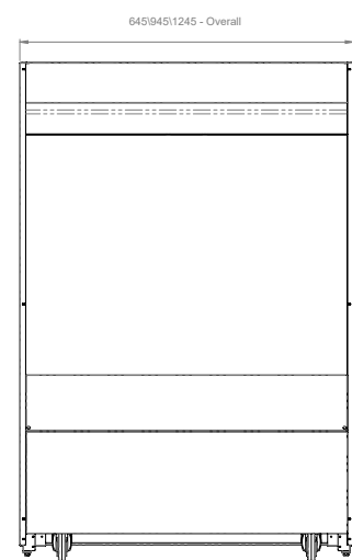
Rear Elevation
