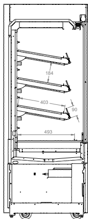
Section Elevation
