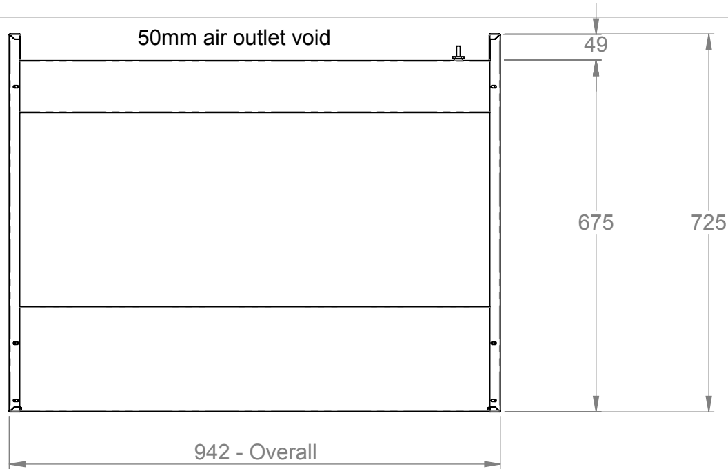
Plan
