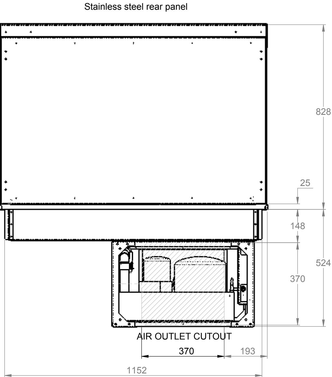
Rear elevation
