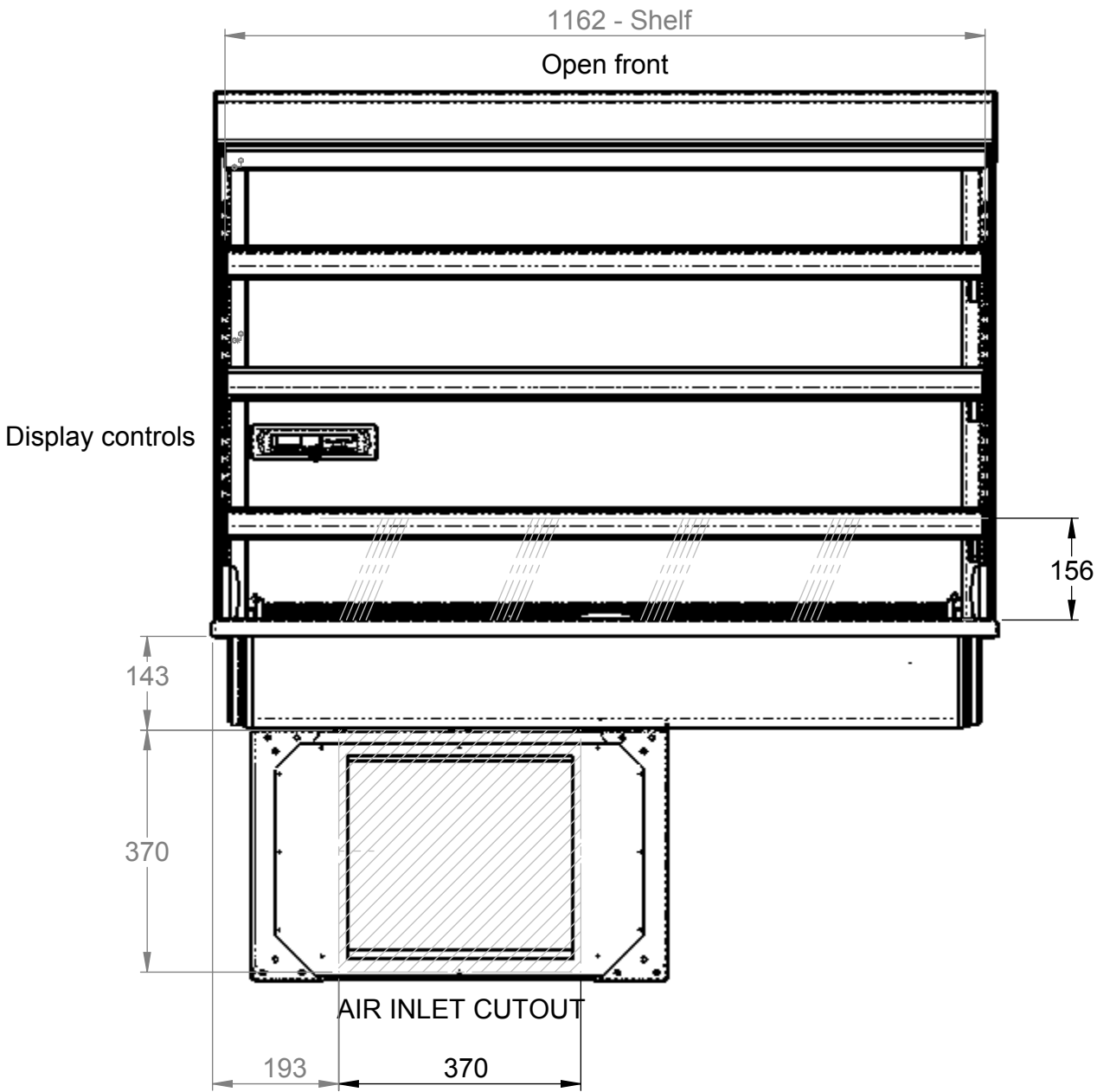
Front elevation
