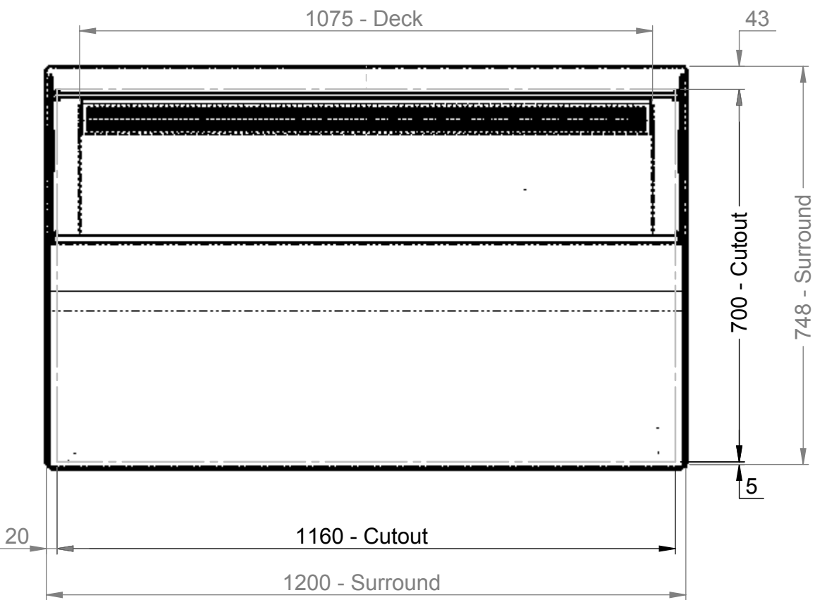
Plan
