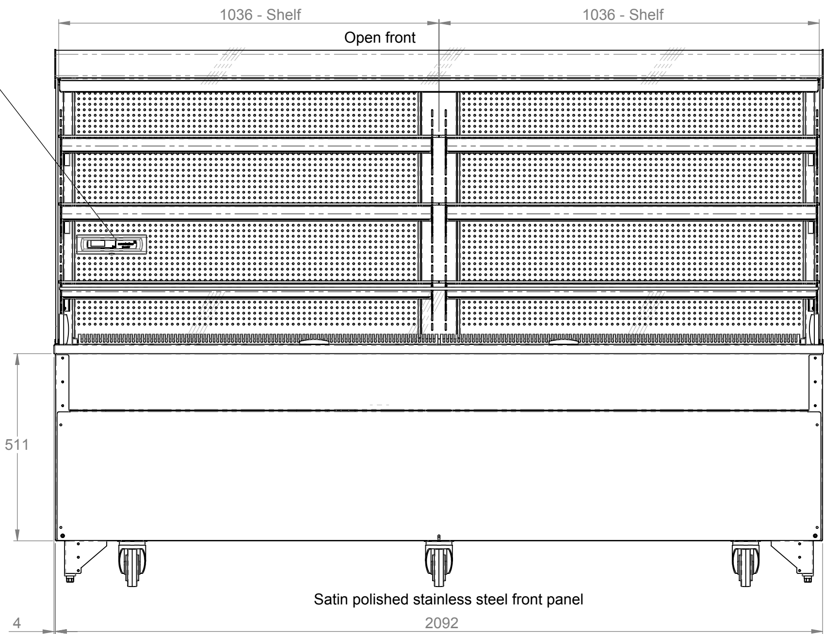
Front elevation
