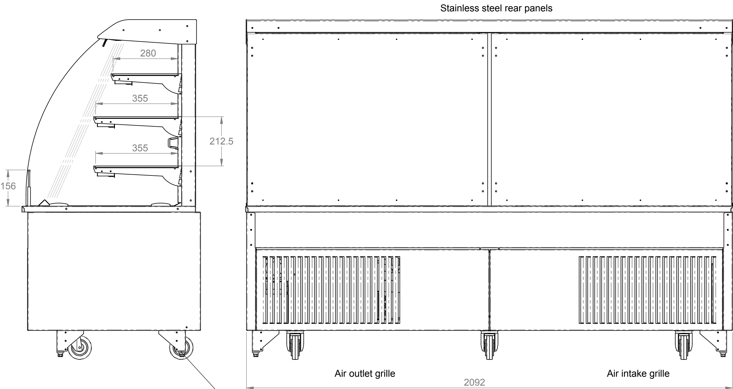
Rear elevation
