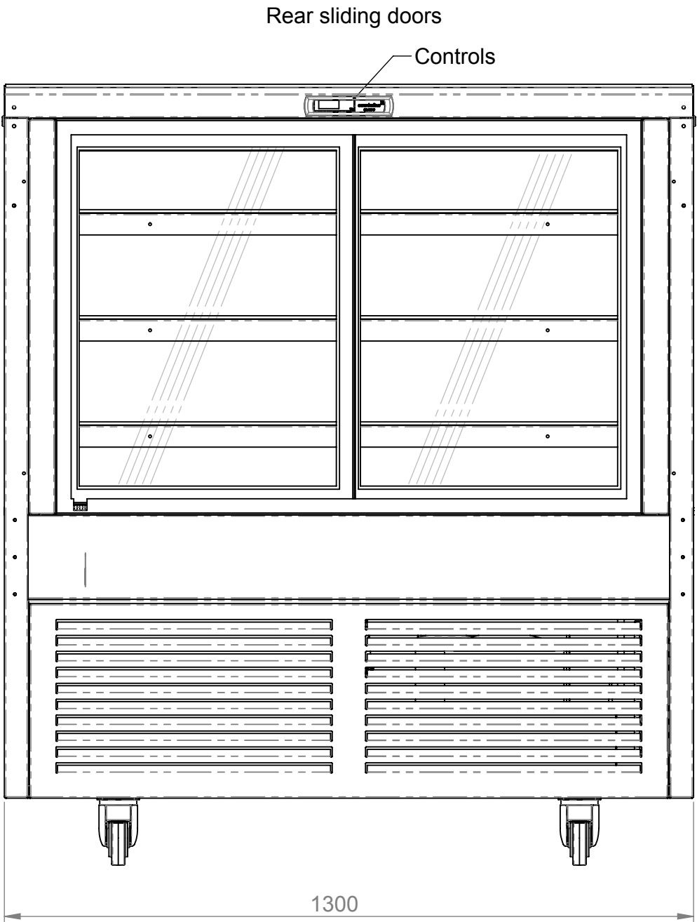
Rear elevation
