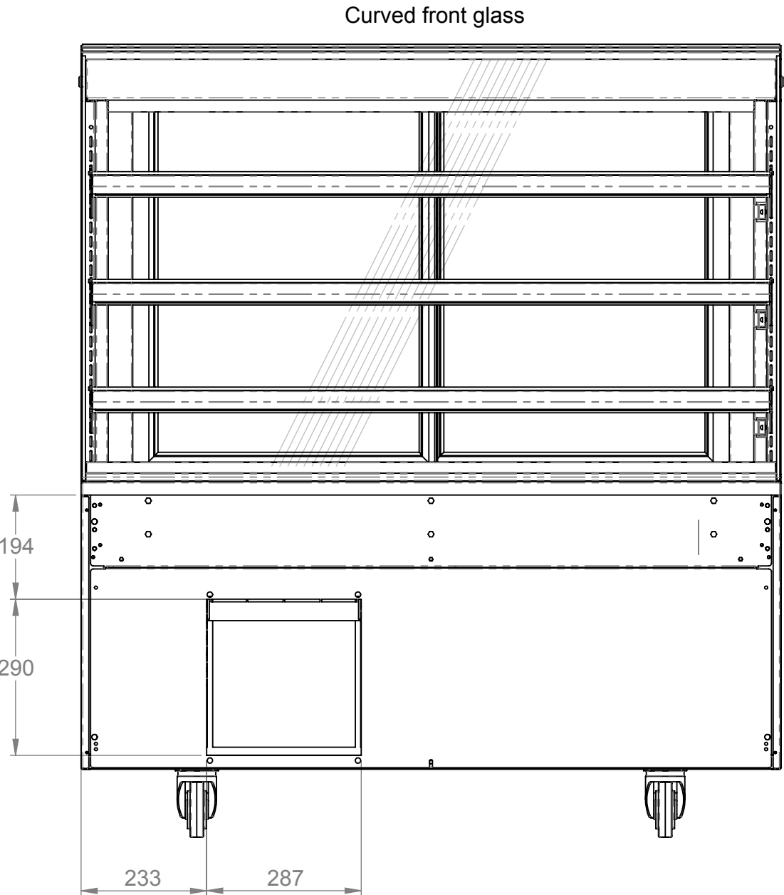
Front elevation
