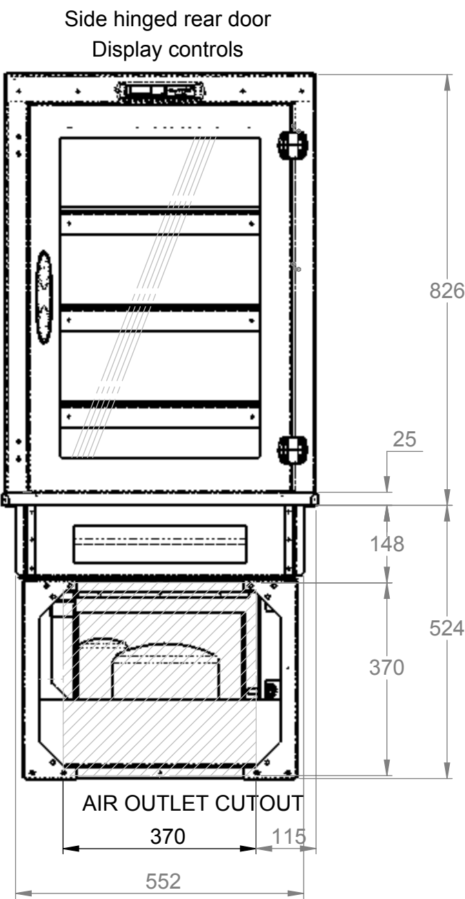
Rear elevation
