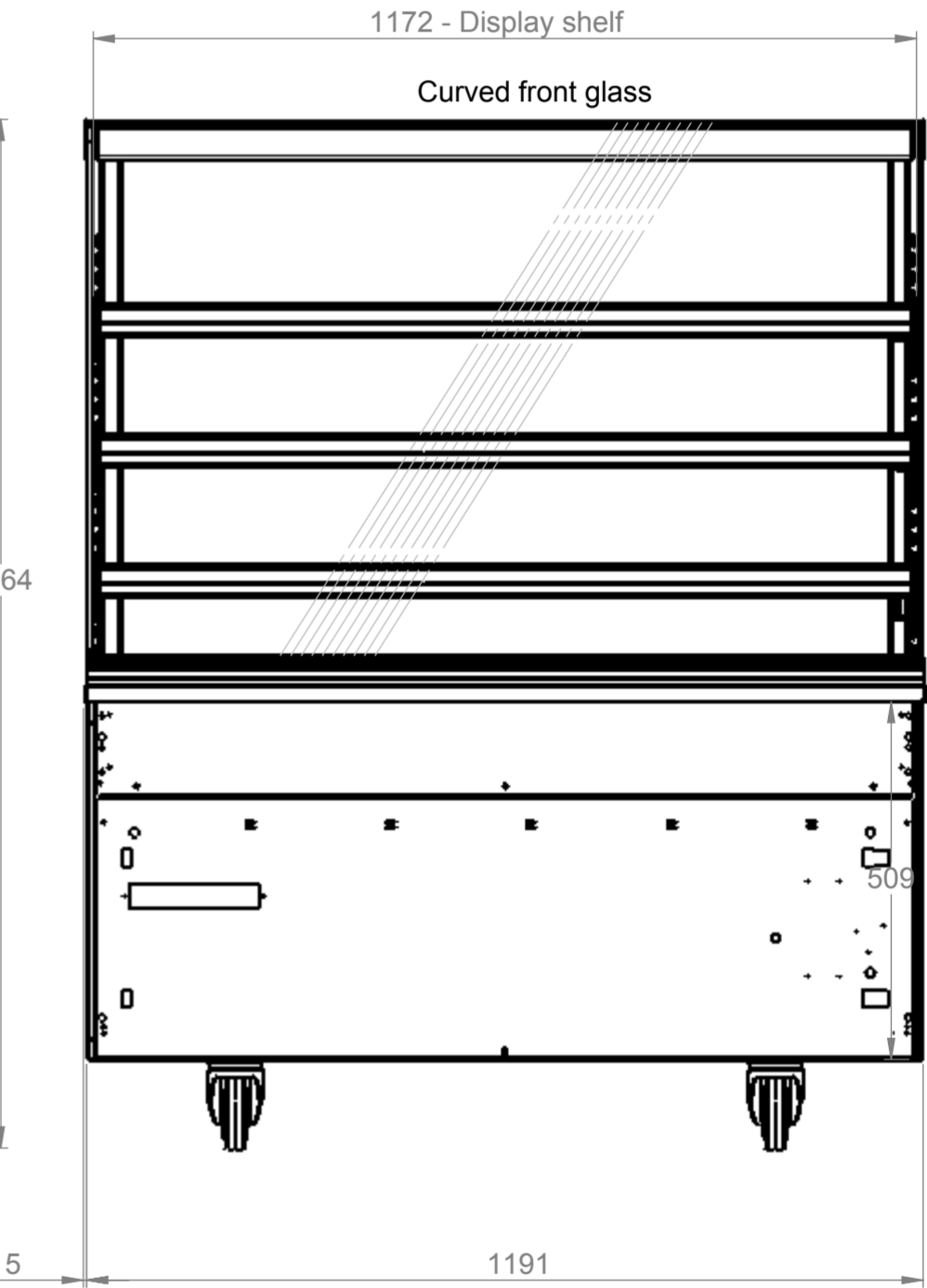
Front elevation
