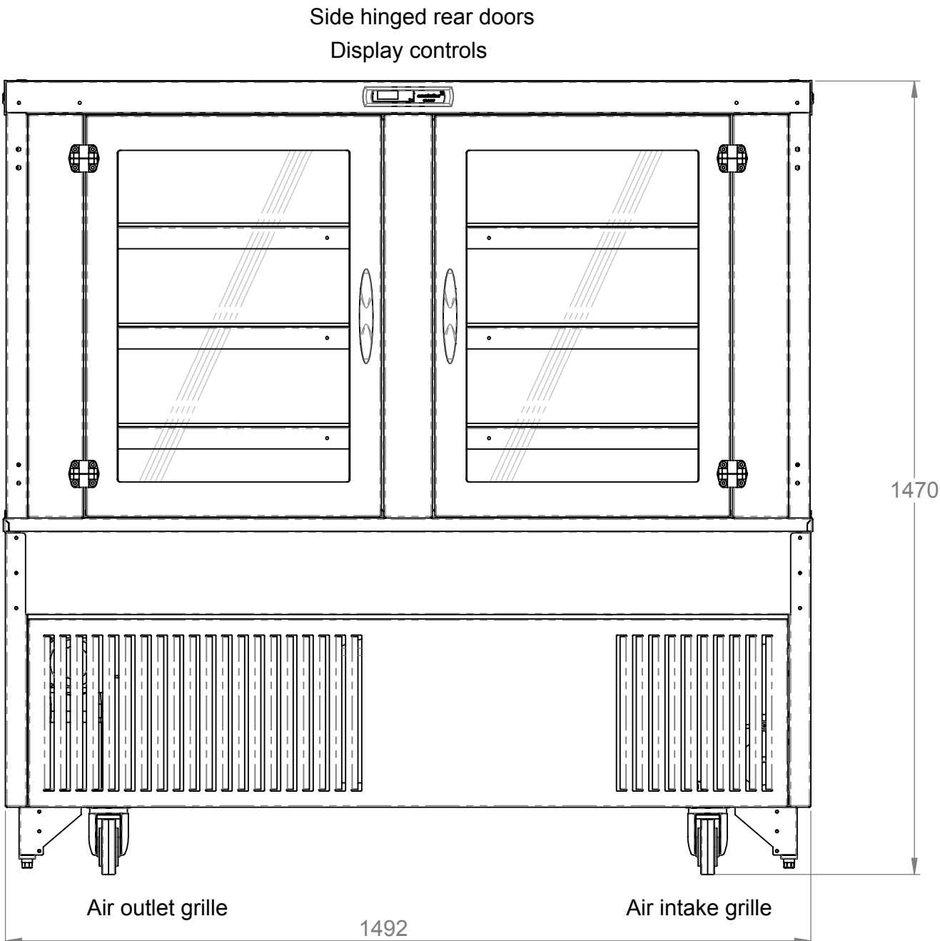
Rear elevation
