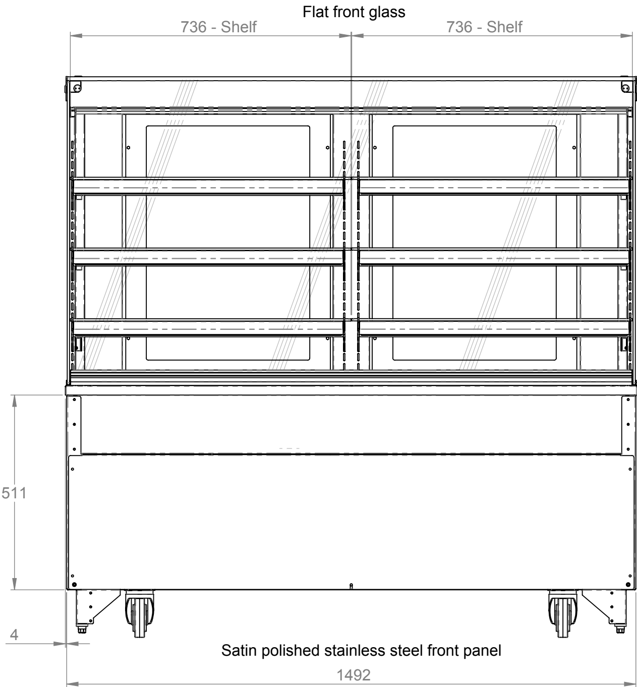
Front elevation
