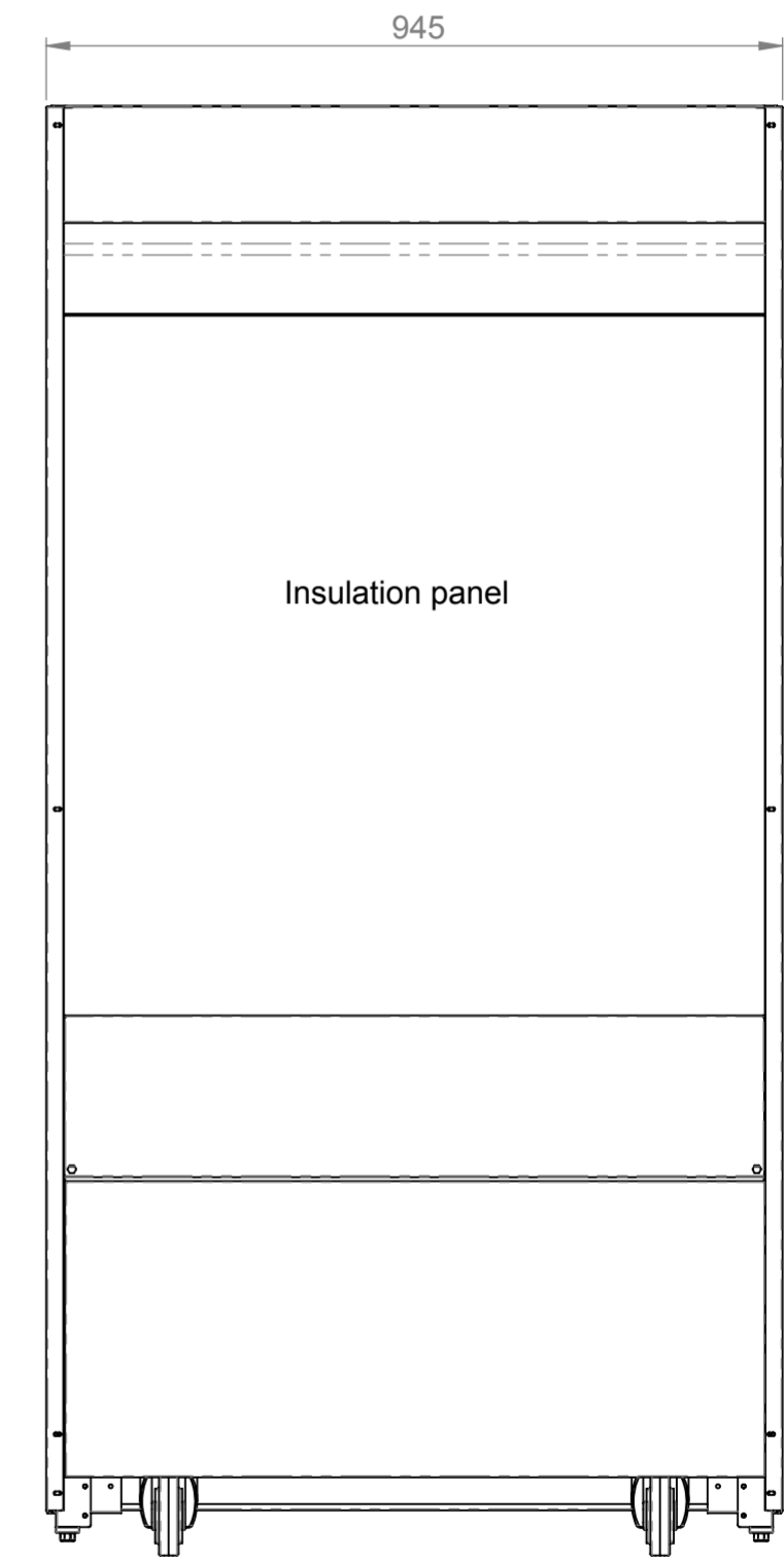
Rear elevation
