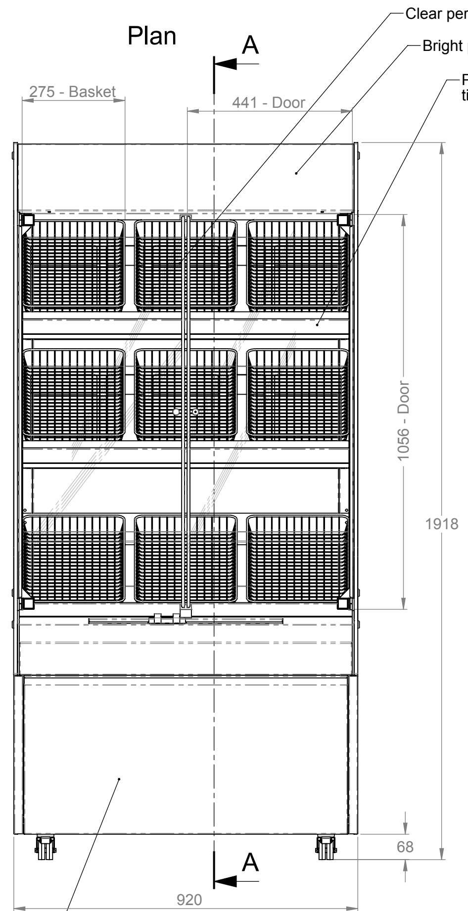
Front elevation
