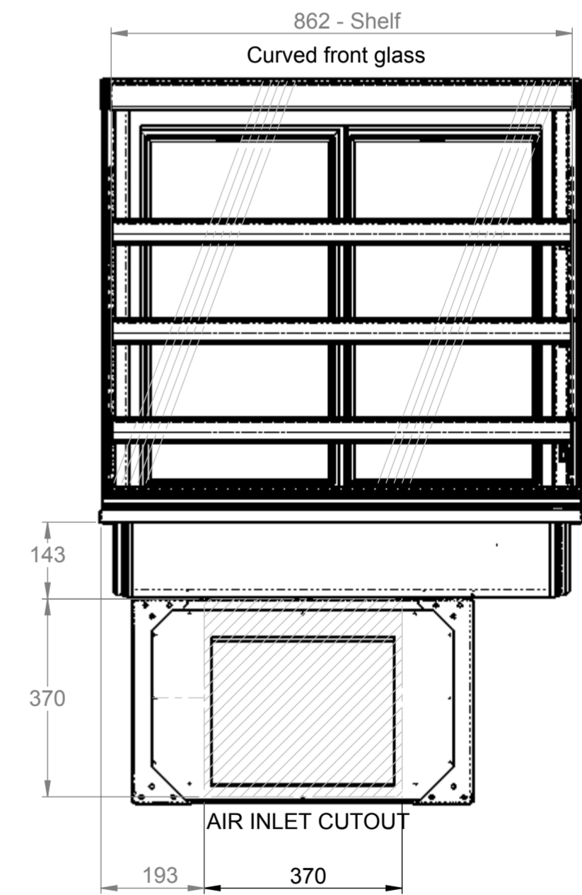
Front elevation
