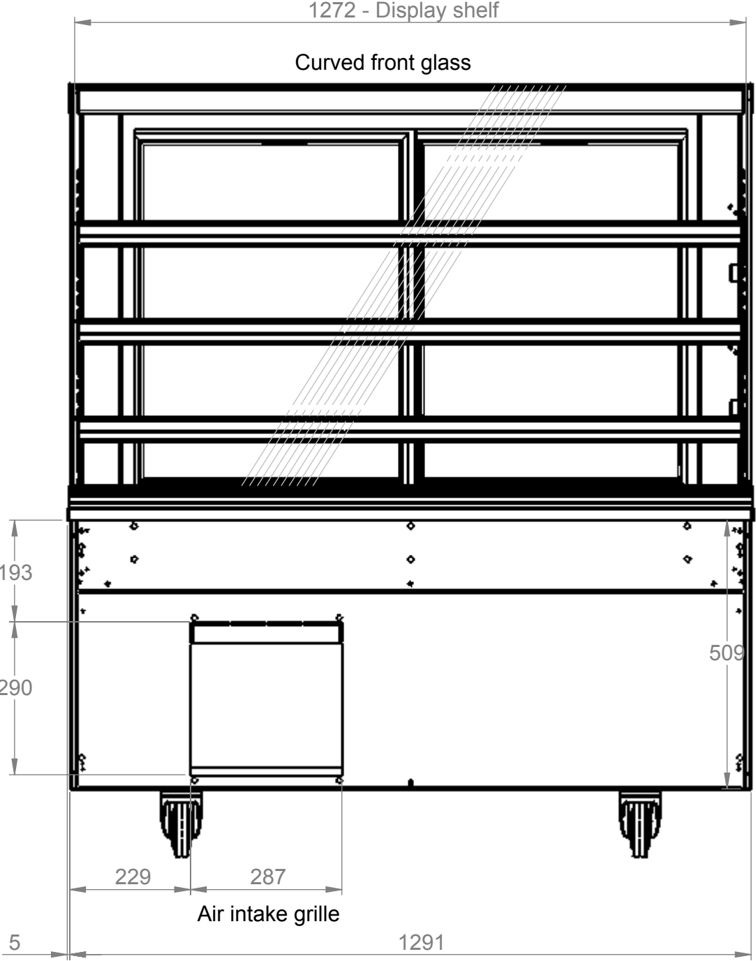
Front elevation
