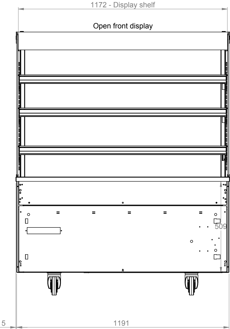
Front elevation
