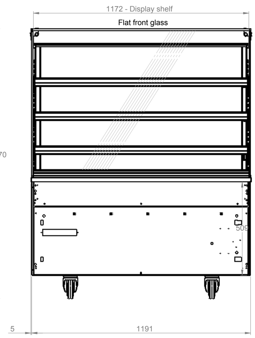
Front elevation
