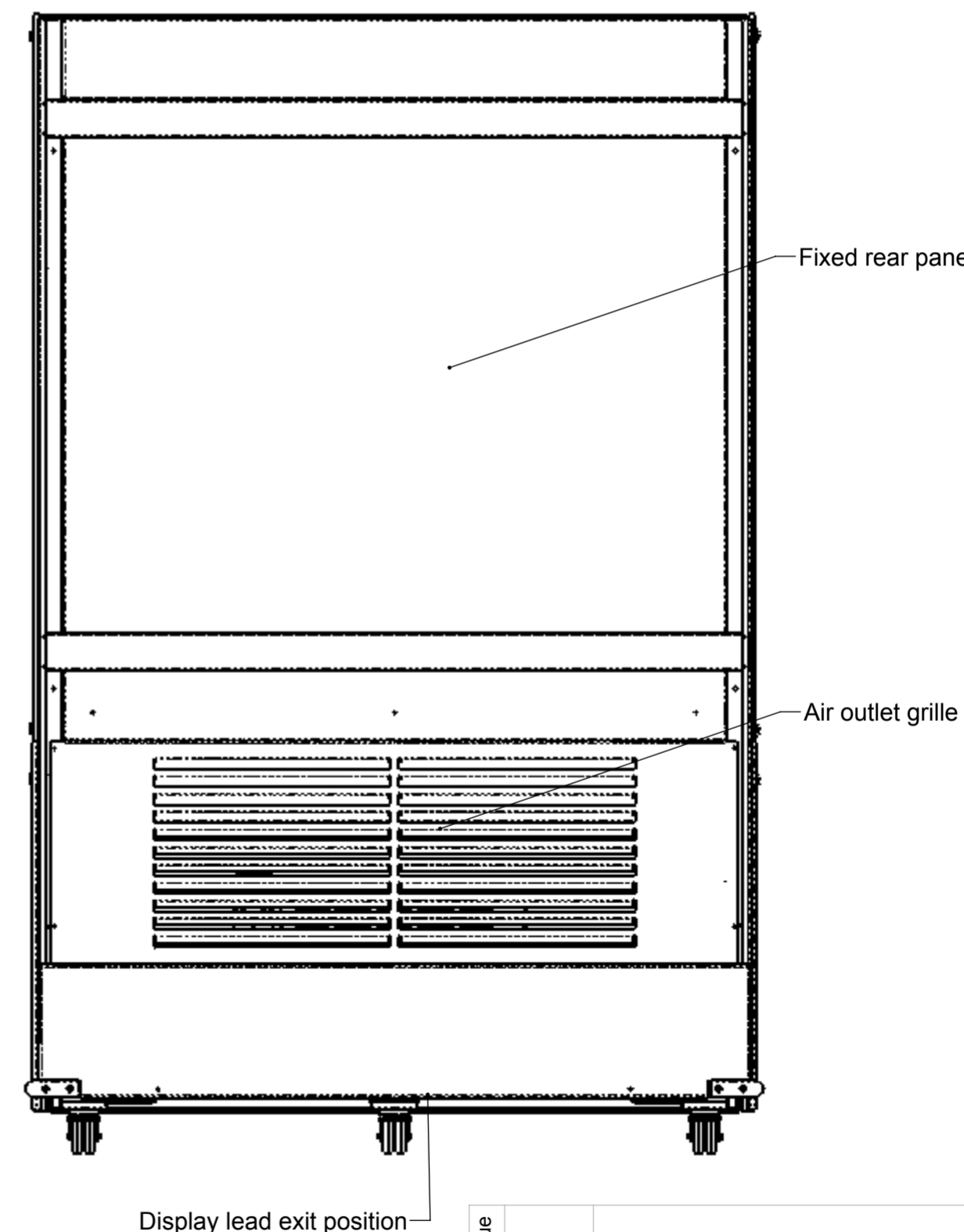
Rear elevation
