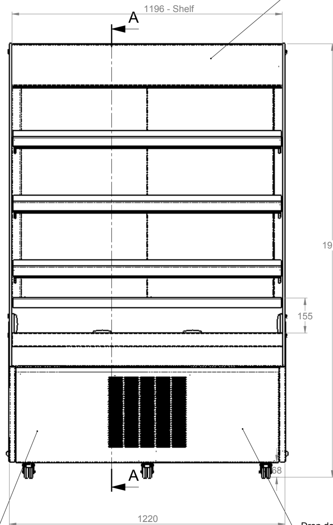
Front elevation
